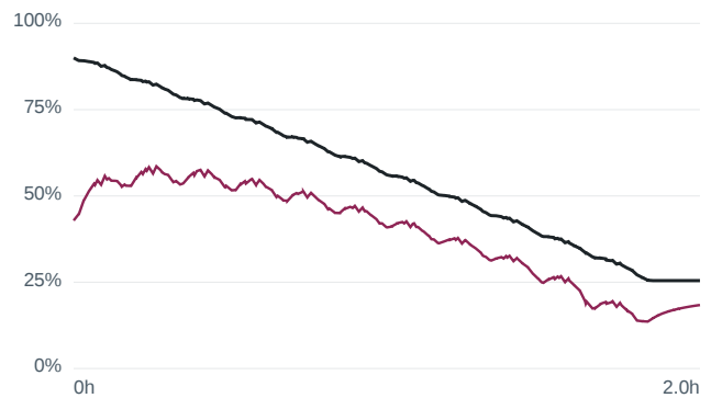
Wrong initial SOC 90 % — m80 US06 at -1... RMSE 18.66 %
