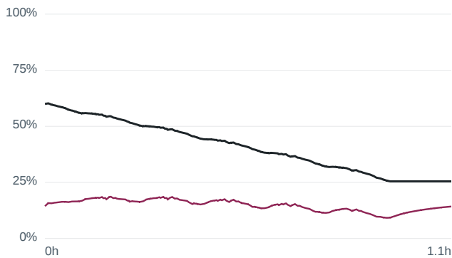
Wrong initial SOC 60 % — m80 US06 at -1... RMSE 27.43 %
