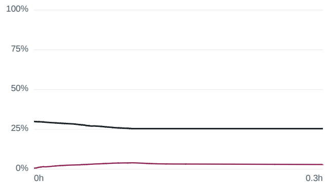
Wrong initial SOC 30 % — m80 US06 at -1... RMSE 23.26 %
