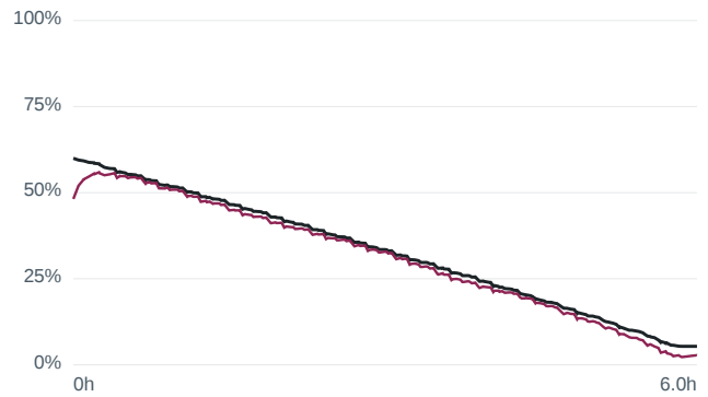
Wrong initial SOC 60 % — m80 LA92 at 25... RMSE 1.95 %
