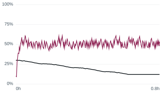
Wrong initial SOC 30 % — m80 US06 at 1... RMSE 32.39 %
