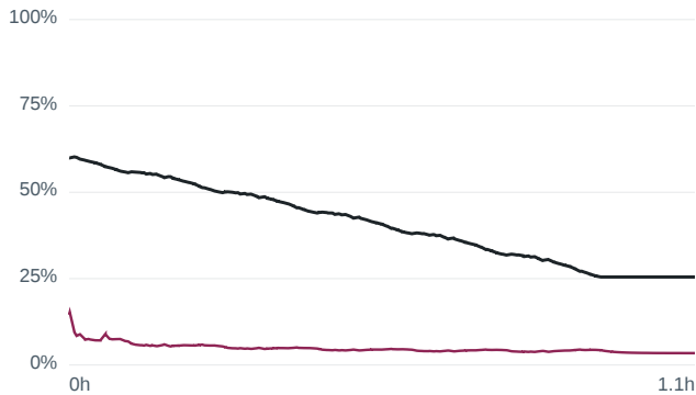
Wrong initial SOC 60 % — m80 US06 at -1... RMSE 37.32 %
