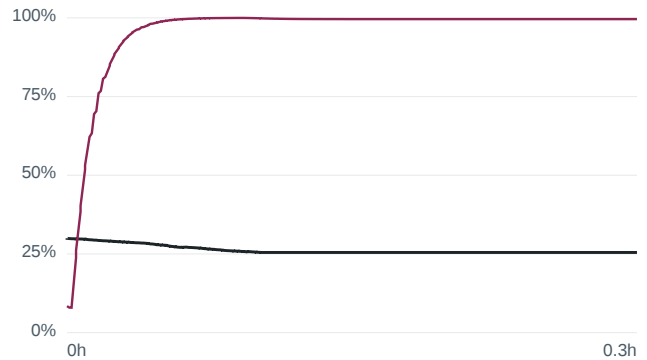
Wrong initial SOC 30 % — m80 US06 at -1... RMSE 70.90 %
