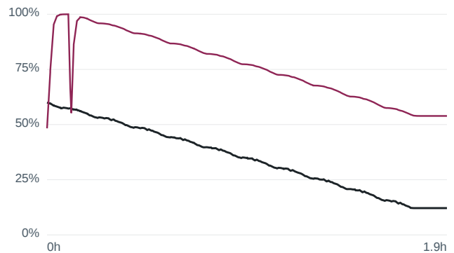
Wrong initial SOC 60 % — m80 US06 at 1... RMSE 41.90 %
