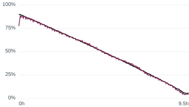
Wrong initial SOC 90 % — m80 LA92 at 25... RMSE 1.24 %
