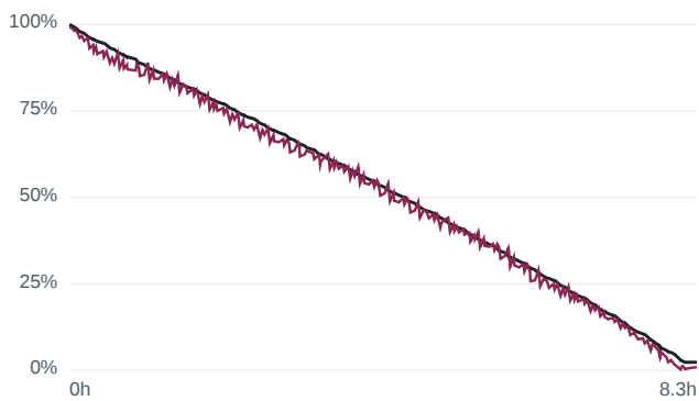
Current-sensor offset +0.3 A — m1000... RMSE 2.01 %
