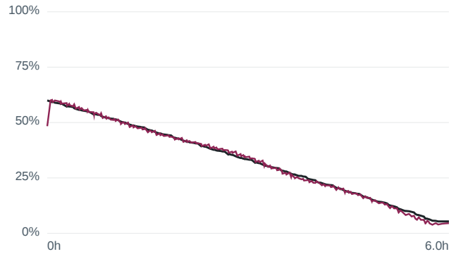
Wrong initial SOC 60 % — m80 LA92 at 25... RMSE 1.19 %
