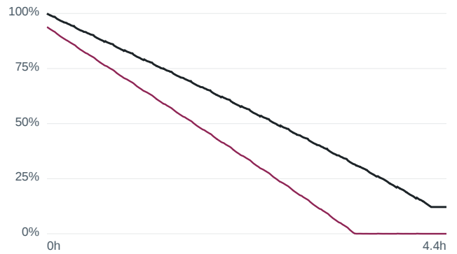
Current-sensor offset -0.3 A — m1000... RMSE 20.35 %
