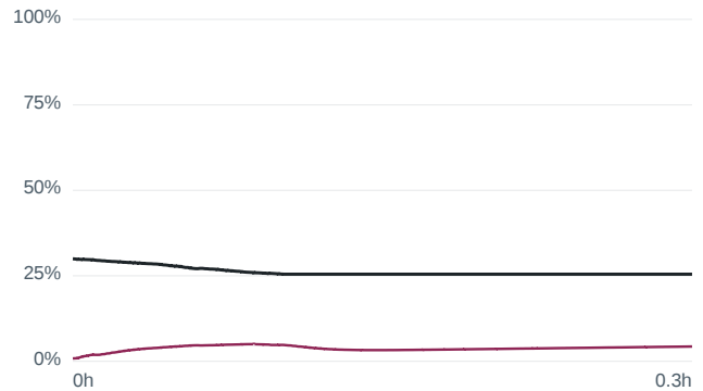
Wrong initial SOC 30 % — m80 US06 at -1... RMSE 22.54 %
