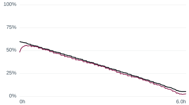
Wrong initial SOC 60 % — m80 LA92 at 25... RMSE 1.95 %
