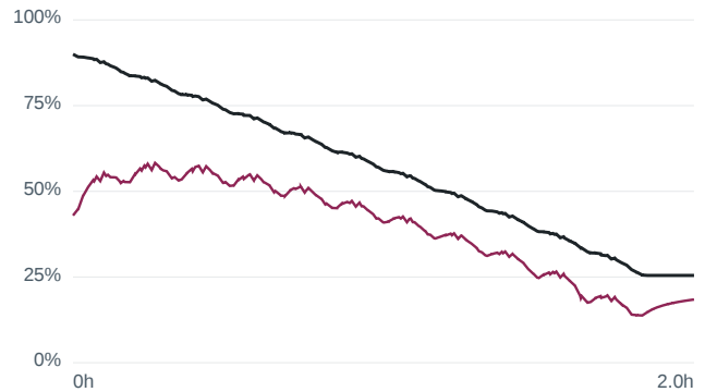
Wrong initial SOC 90 % — m80 US06 at -1... RMSE 18.72 %
