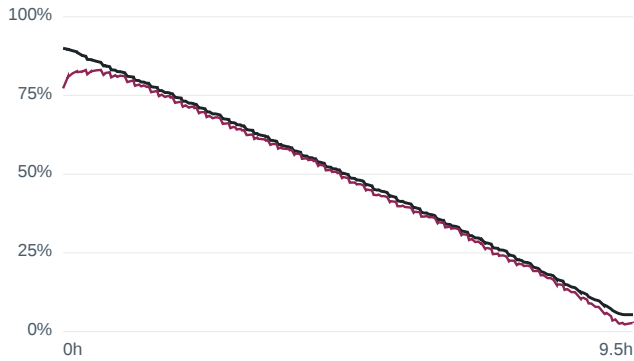
Wrong initial SOC 90 % — m80 LA92 at 25... RMSE 2.17 %
