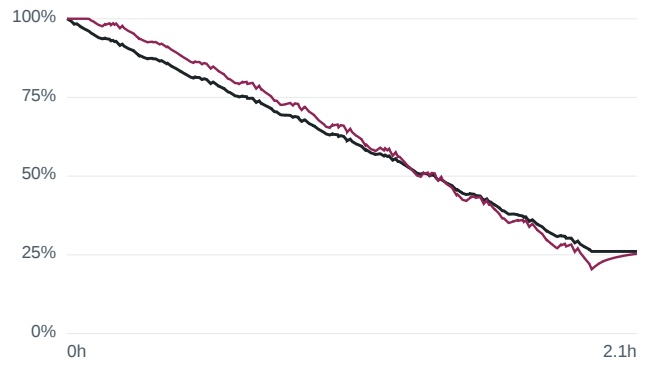
Current-sensor offset -0.3 A — m1000... RMSE 3.49 %
