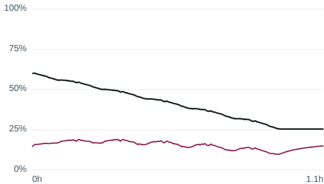
Wrong initial SOC 60 % — m80 US06 at -1... RMSE 26.96 %
