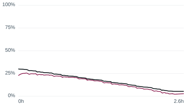
Wrong initial SOC 30 % — m80 LA92 at 25... RMSE 2.42 %
