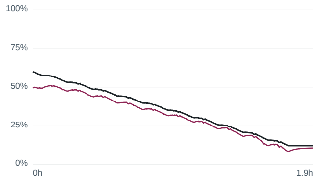
Wrong initial SOC 60 % — m80 US06 at 1... RMSE 3.99 %
