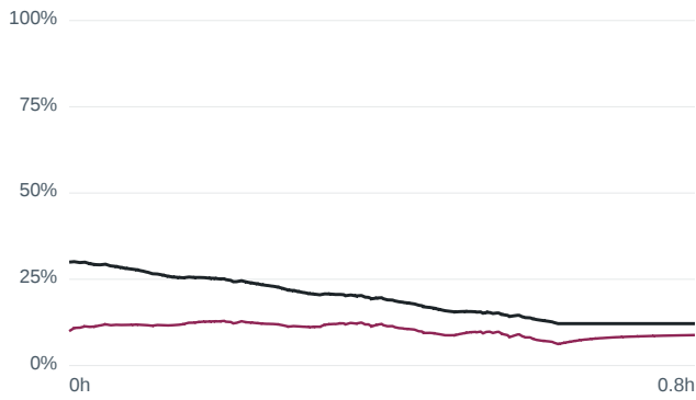
Wrong initial SOC 30 % — m80 US06 at 1... RMSE 10.06 %
