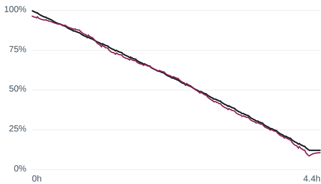
Current-sensor offset +0.3 A — m1000... RMSE 1.43 %
