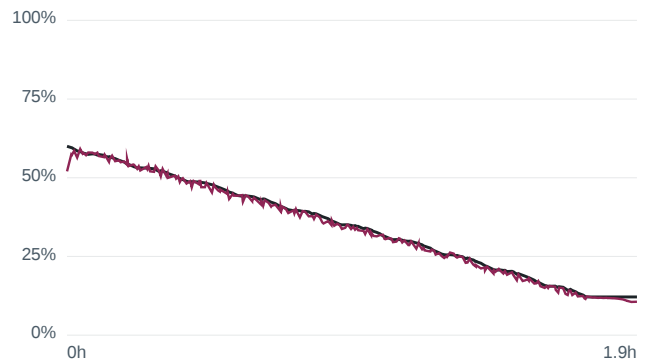
Wrong initial SOC 60 % — m80 US06 at 1... RMSE 1.08 %
