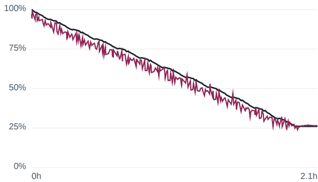
Current-sensor offset +0.3 A — m1000... RMSE 4.35 %
