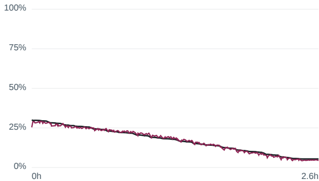
Wrong initial SOC 30 % — m80 LA92 at 25... RMSE 0.92 %
