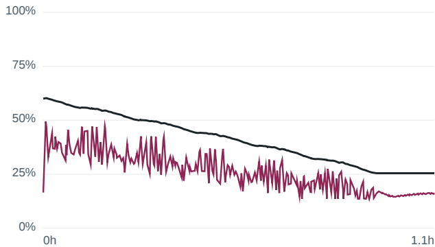
Wrong initial SOC 60 % — m80 US06 at -1... RMSE 15.55 %
