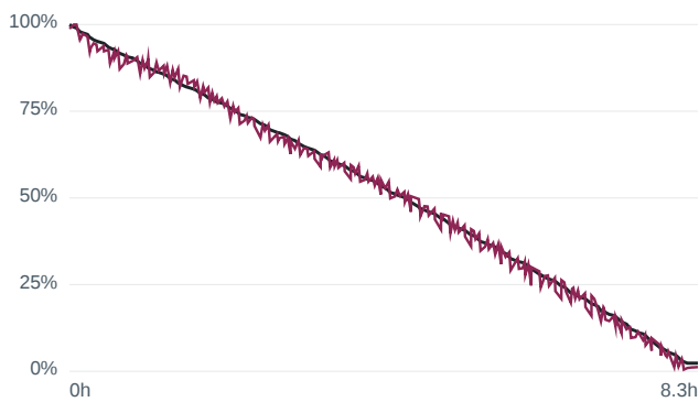
Current-sensor offset +0.3 A — m1000... RMSE 1.89 %
