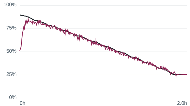
Wrong initial SOC 90 % — m80 US06 at -1... RMSE 4.89 %
