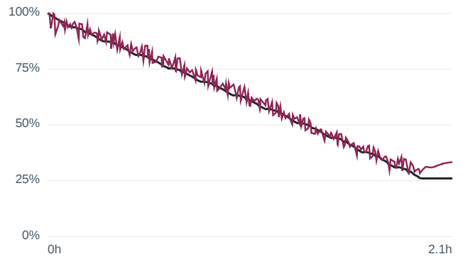
Current-sensor offset -0.3 A — m1000... RMSE 3.01 %
