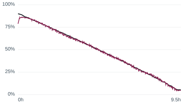
Wrong initial SOC 90 % — m80 LA92 at 25... RMSE 1.32 %
