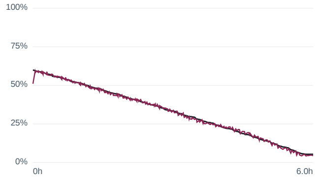
Wrong initial SOC 60 % — m80 LA92 at 25... RMSE 1.04 %
