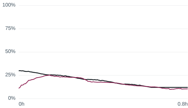
Wrong initial SOC 30 % — m80 US06 at 1... RMSE 4.16 %
