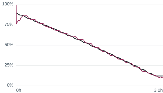
Wrong initial SOC 90 % — m80 US06 at 1... RMSE 1.95 %
