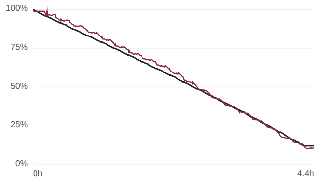
Current-sensor offset -0.3 A — m1000... RMSE 2.38 %
