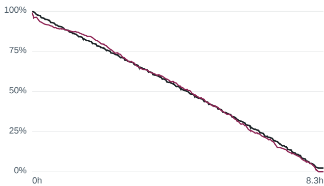
Current-sensor offset +0.3 A — m1000... RMSE 1.69 %
