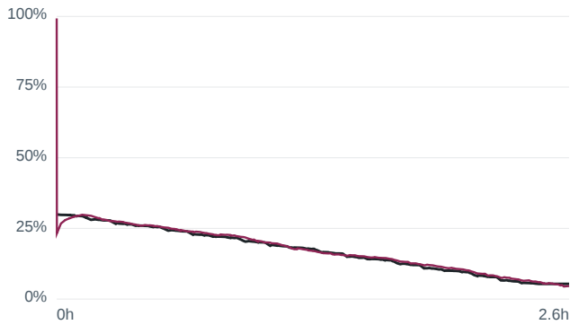
Wrong initial SOC 30 % — m80 LA92 at 25... RMSE 4.55 %
