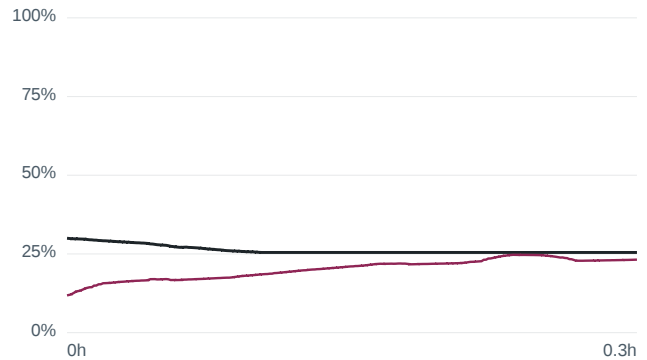
Wrong initial SOC 30 % — m80 US06 at -1... RMSE 7.45 %
