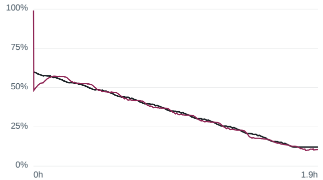
Wrong initial SOC 60 % — m80 US06 at 1... RMSE 3.10 %
