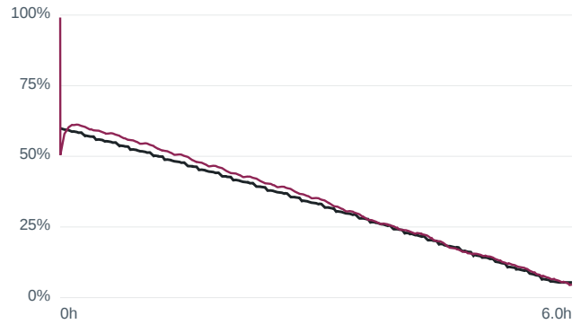
Wrong initial SOC 60 % — m80 LA92 at 25... RMSE 3.17 %
