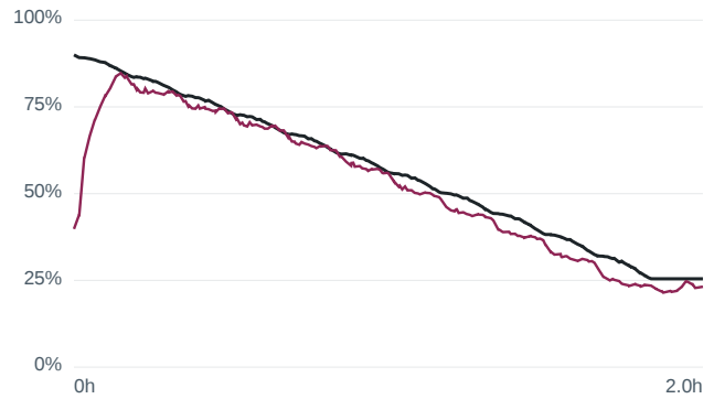
Wrong initial SOC 90 % — m80 US06 at -1... RMSE 7.31 %
