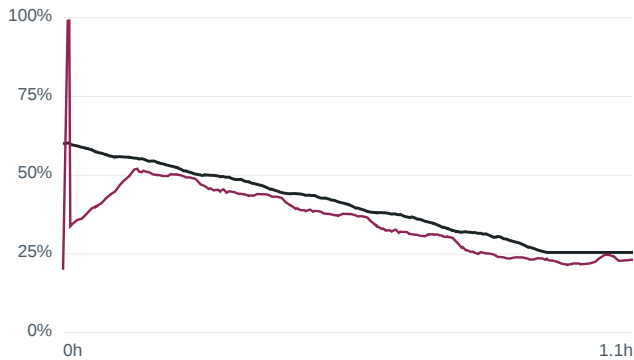
Wrong initial SOC 60 % — m80 US06 at -1... RMSE 8.00 %
