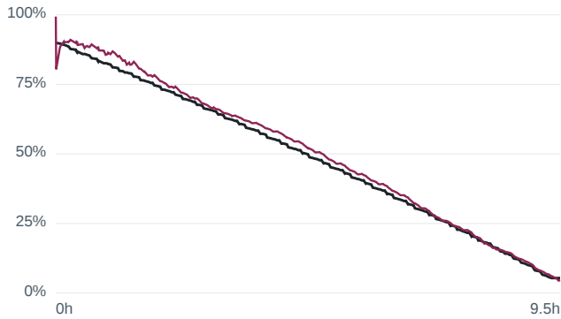
Wrong initial SOC 90 % — m80 LA92 at 25... RMSE 2.43 %
