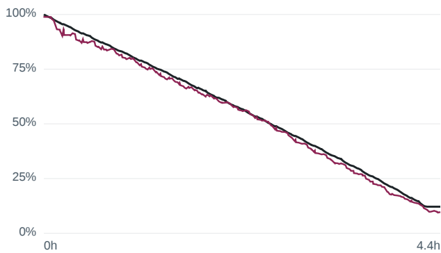
Current-sensor offset +0.3 A — m1000... RMSE 2.11 %
