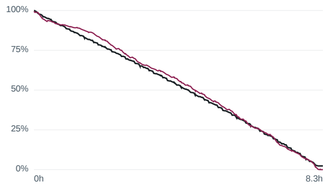
Current-sensor offset -0.3 A — m1000 LA... RMSE 2.41 %
