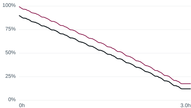
Wrong initial SOC 90 % — m80 US06 at 1... RMSE 7.78 %
