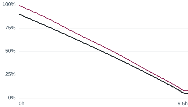
Wrong initial SOC 90 % — m80 LA92 at 25... RMSE 6.20 %
