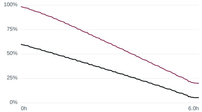
Wrong initial SOC 60 % — m80 LA92 at 25... RMSE 28.44 %
