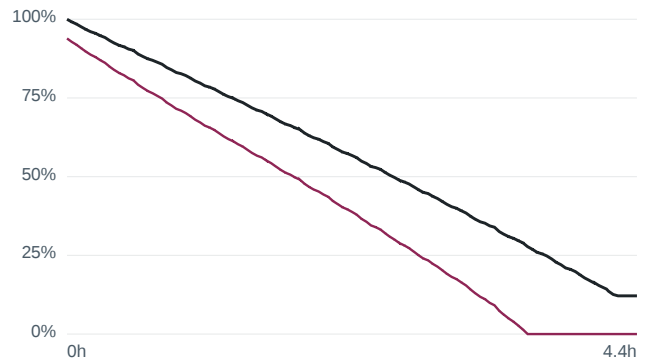
Current-sensor offset -0.3 A — m1000... RMSE 22.05 %
