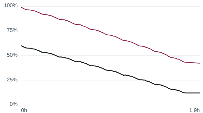
Wrong initial SOC 60 % — m80 US06 at 1... RMSE 35.61 %
