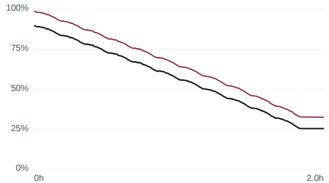
Wrong initial SOC 90 % — m80 US06 at -1... RMSE 8.23 %
