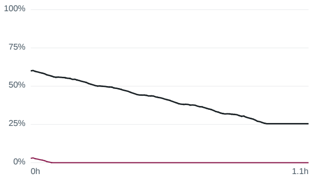
Wrong initial SOC 60 % — m80 US06 at -1... RMSE 47.23 %
