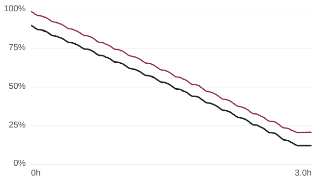
Wrong initial SOC 90 % — m80 US06 at 1... RMSE 8.04 %
