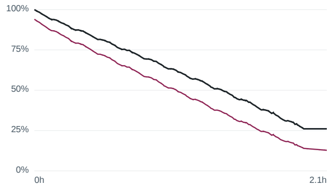
Current-sensor offset -0.3 A — m1000... RMSE 11.49 %
