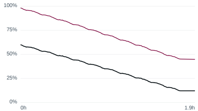
Wrong initial SOC 60 % — m80 US06 at 1... RMSE 35.38 %
