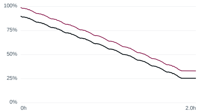
Wrong initial SOC 90 % — m80 US06 at -1... RMSE 8.30 %
