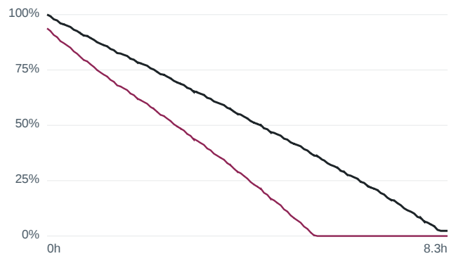
Current-sensor offset -0.3 A — m1000 LA... RMSE 23.93 %
