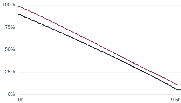
Wrong initial SOC 90 % — m80 LA92 at 25... RMSE 6.27 %
