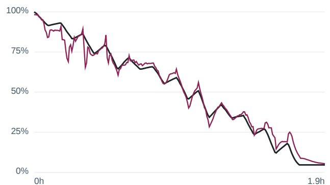
m1000 HWGRADE at 25 °C
